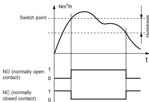
Fig. 2 Hysteresis mode
