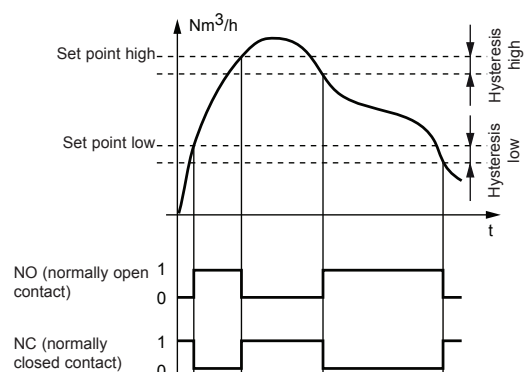
Fig. 3 Window mode
